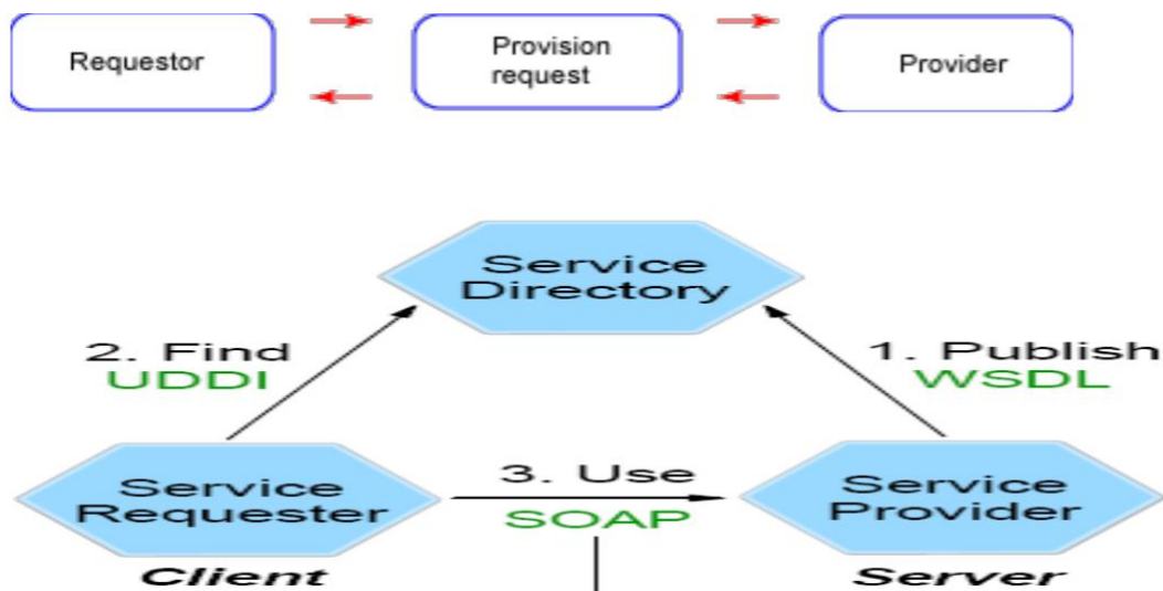
Figure 1: Web services Architecture
