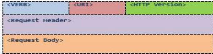
Figure 1: HTTP request format.
