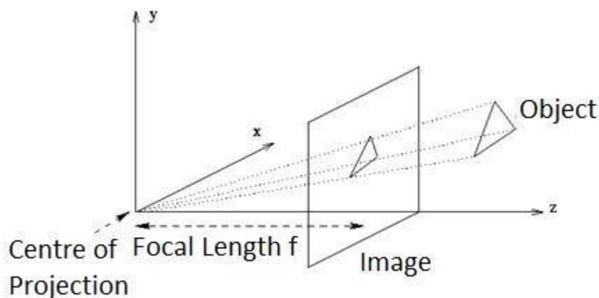
Fig. 4.2: - perspective projection
