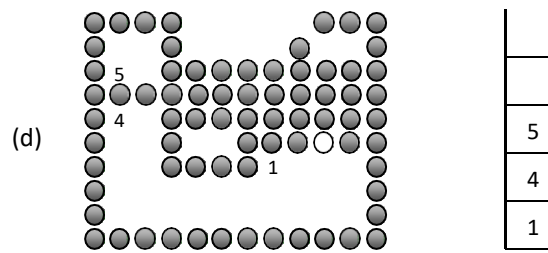
Fig. 2.24: - Boundary fill across pixel spans for a 4-connected area.
