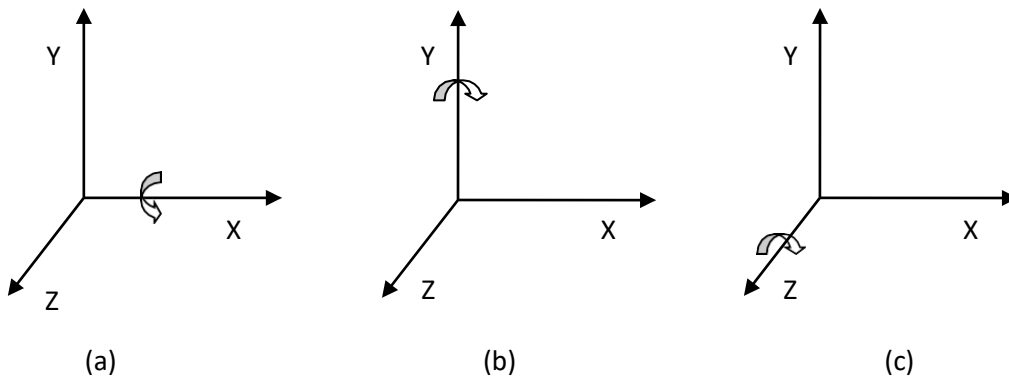
Fig. 5.2: - 3D Rotations.
