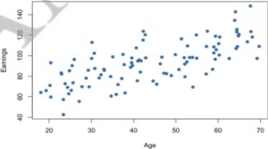
A Scatterplot of X and Y
